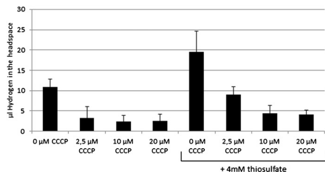
Fig. 5. Role of uncoupler, CCCP, in the sulfur and thiosulfate driven H_2 evolution in THOE5M strain. The H_2 evolution was monitored in the presence of endogenous elemental sulfur and additives. The examined period was only one day due to the spontaneous decomposition of CCCP and the experiments were performed in smaller volume with fewer cells than in the previous experiments. Therefore, the absolute values of the H_2 content cannot be compared to the data shown in other figures.
