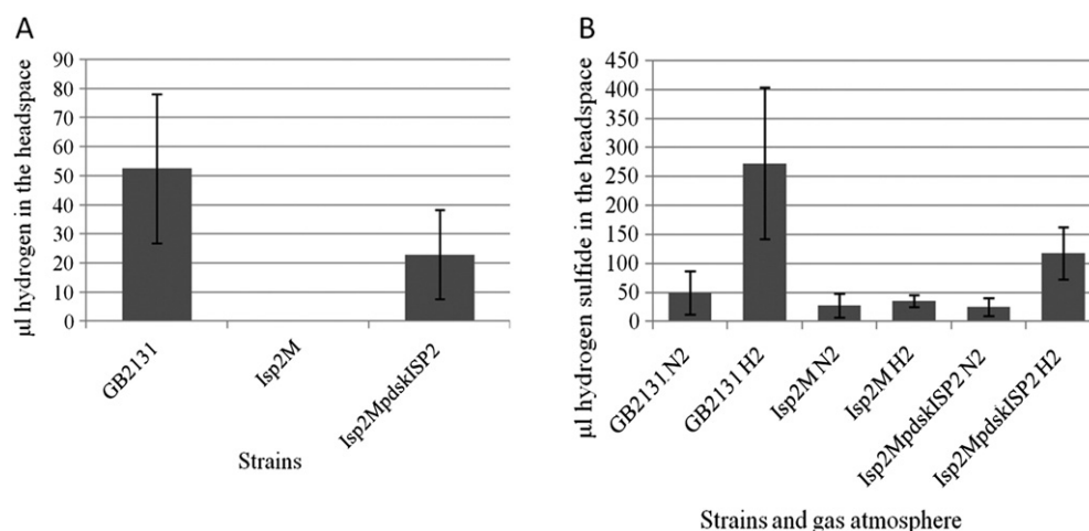
Fig. 4. Effect of isp2 deletion on the HynSL-linked A) H_2 evolution, B) H_2 -driven H_2S formation. H_2S production of cultures was monitored in the presence of elemental sulfur under N_2 or H_2 atmosphere (indicated in the label of x axis). For the names of the strains see Table 1. For the details of the experiments see Materials and Methods.
